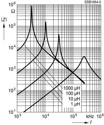
Impedance |Z| versus frequency f measured with impedance analyzer HP 4291A; test fixture 16193A
